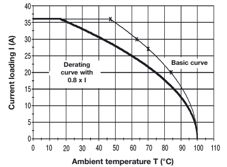
TOP4GS/6/6.35 with Conductor H07V-K4.0 mm 2
